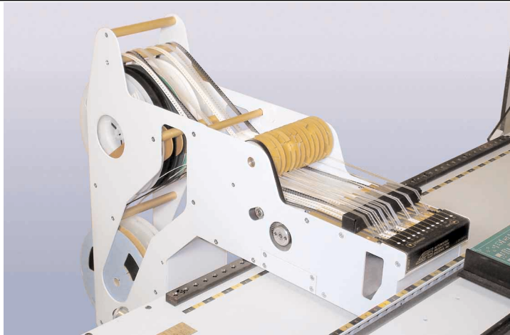
Model L-GB-12 Bank Feeder
